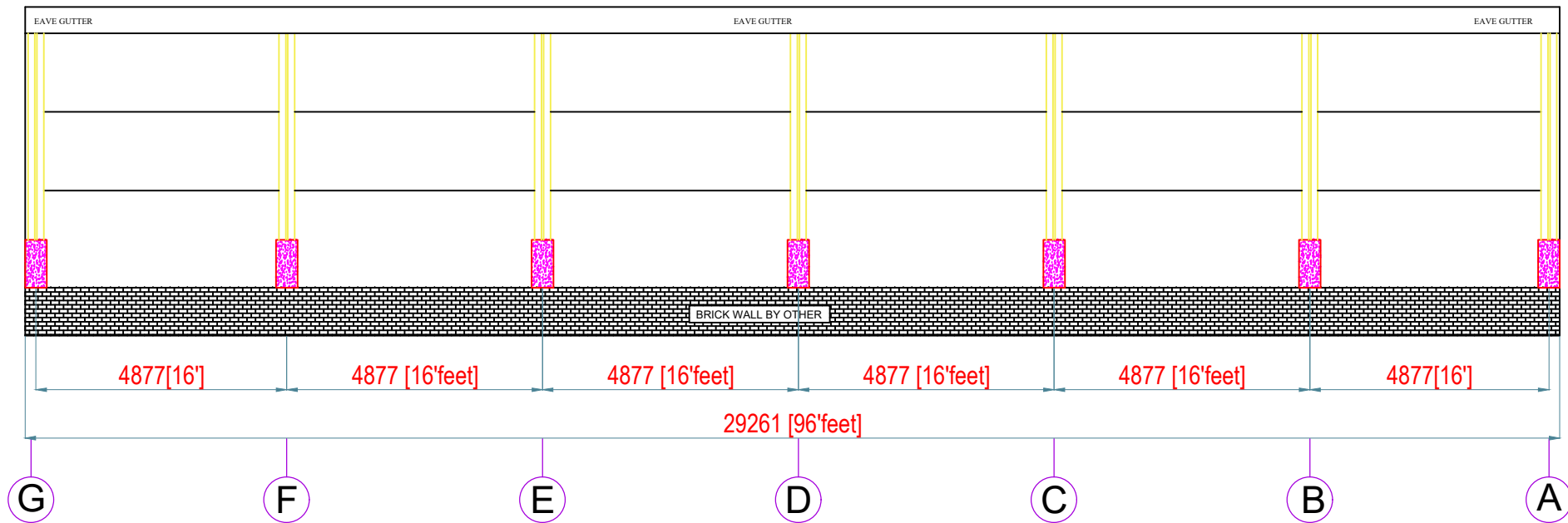
SIDE WALL FRAMING @ GL 6
